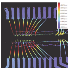
Wirebond inspection
